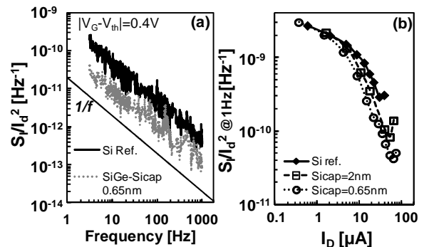
Fig. 11: (a) SiGe devices with a reduced Si cap thickness for optimized NBTI reliability also show reduced 1/f noise w.r.t. a Si ref. device with identical gate-stack, (b) and also with respect to a SiGe device with thicker Si cap.
