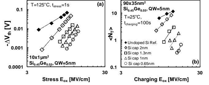
Fig. 5: (a) Large area devices: SiGe channel pMOSFETs with a reduced Si cap thickness show reduced NBTI \Delta V_{th} and a stronger field acceleration leading to further improvement at lower operating fields. (b) Nanoscaled devices: the same experimental observations apply to the average number of charging/discharging defects per device ( \langle N_T \rangle ). Note: very high equivalent oxide fields were needed for the preliminary charging phase in order to be able to observe active defects in SiGe devices with the thinnest Si cap ( \langle N_T \rangle as low as \sim 0.33 at 15MV/cm, i.e. one defect observed for every 3 measured devices).
