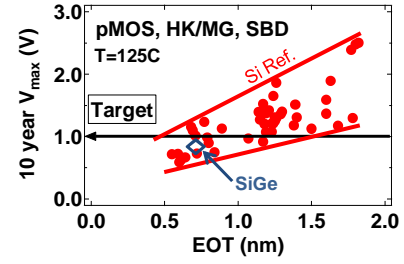
Fig. 14: Extracted maximum operating gate voltage using a soft breakdown (i.e. non-destructive) failure criterion for a \sim 0.7 nm EOT NBTI-optimized SiGe gate stack shows no difference with respect to Si channel device benchmark data [30].
