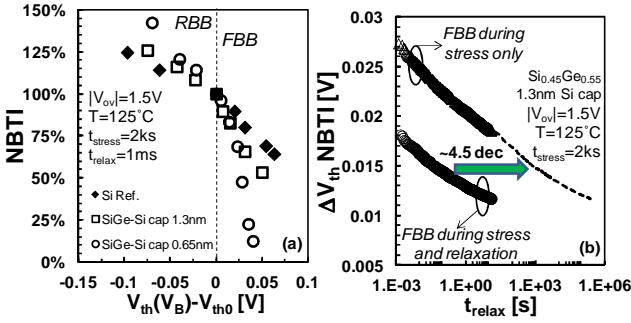
Fig. 12: (a) The body bias is found to modulate the oxide electric field at a given overdrive gate voltage and therefore the NBTI degradation. Due to the stronger electric field dependence of NBTI observed in SiGe pMOSFETs with reduced Si cap thickness (Fig. 5), more reduced NBTI with FBB is observed. (b) A significantly faster NBTI relaxation is observed when a FBB is applied during an entire stress/relaxation sequence.
