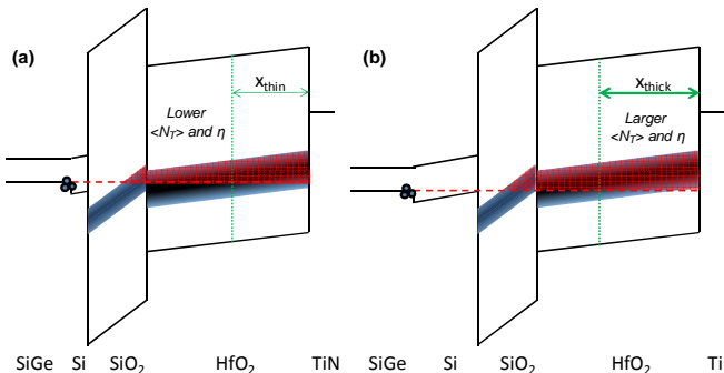
Fig. 10: Sketches of the SiGe gate stacks in the stress condition, showing the defect bands in the SiO 2 and HfO 2 as from the model proposed in Part I for large area devices. Thanks to the higher Fermi level in the SiGe channel, fewer defects are energetically favorable for channel holes. Moreover the accessible defects are preferentially spatially located further from the channel, toward the gate, yielding a reduction of \eta . (a) The favorable alignment shift is maximized for the thinnest Si cap thickness, while (b) the additional voltage drop on a thicker Si cap (at fixed field) makes more defects on the channel side accessible, displacing the equivalent trapped charge centroid ( x_{thick} > x_{thin} ). This observation readily explains the larger \langle N_T \rangle and \eta observed for SiGe devices with thick Si caps.
