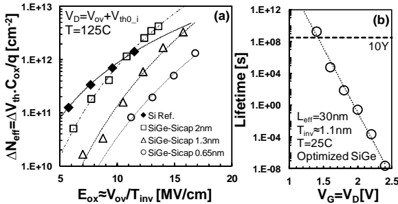
Fig. 13: (a) SiGe devices with a thick Si cap show lower CHC degradation w.r.t. Si ref. only at low stress conditions, while at high stress conditions a higher degradation is apparent probably due to enhanced impact ionization in the small bandgap channel. However, the optimized SiGe gate-stacks with a reduced Si cap thickness consistently show an overall reduced CHC degradation w.r.t. Si ref. (b) Extrapolated device lifetime under CHC stress for a \sim 0.7 nm EOT ( T_{inv} \approx 1.1 nm) NBTI-optimized SiGe gatestack. CHC do not constitute a showstopper for SiGe devices.
