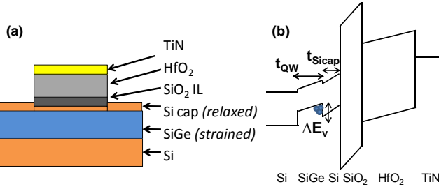
Fig. 1 (a) Sketch of the gate stack of SiGe devices used in this work. (b) Band diagram in inversion: channel holes are confined into the SiGe QW due to the valence band offset ( \Delta E_v ) between the SiGe channel and the Si cap.
