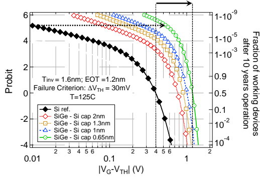
Fig. 9: Calculated fractions of working devices after 10 year continuous operation at varying operating voltages for the different gate stacks studied here. A dramatic improvement of the distributions is apparent for SiGe devices with reduced Si cap thickness. Note: large area device lifetime would appear in this plot as a vertical dashed line (whole population fails above maximum allowed operating voltage, while it passes for lower voltages) with same median value (Probit=0) of the respective nanoscaled device distribution. The reliability improvement previously observed in large area SiGe devices (demarcated by the solid arrow, distance at Probit=0) is expected to be magnified at high percentiles (demarcated by the dotted arrow, at \sim 1 ppb).
