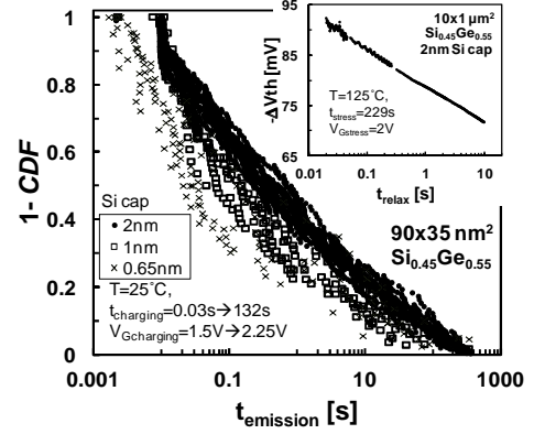
Fig. 8: 1-CDF plot of all the charge emission times observed on multiple devices/traps after preliminary charging phases of different durations and at several voltages, on SiGe gate stacks varying Si cap thickness. The apparent distributions are reminiscent of the NBTI relaxation traces typically observed on large area devices (inset, \Delta V_{th} relaxation trace for a 10 \times 1 \mu\text{m}^2 SiGe device with a 2 nm Si cap). The emission time distributions appear shifted toward lower values for reducing Si cap thicknesses, suggesting a faster discharge of the trapped charges after stress removal, as previously observed for large area devices in [1]. NB: A detailed study of a single trap emission times distribution can be found in [10].
