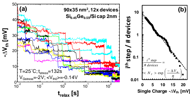
Fig. 2: (a) NBTI relaxation transients recorded on nanoscaled SiGe devices. For each device, multiple single defect discharge events are visible. (b) Weighted complementary Cumulative Distribution Function (CCDF) plot of the individual \Delta V_{th} step heights observed on multiple (41) devices. Despite the intentionally undoped epitaxially grown SiGe channel, the \Delta V_{th} step heights appear to be exponentially distributed [4], with an average value \eta \approx 3.9\text{mV} . The average number of defects per device, \langle N_T \rangle , can be easily read in this plot as the intersection of the distribution with the y-axis [6].
