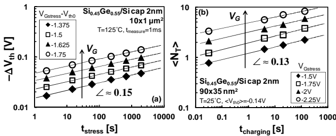
Fig. 4: (a) Large-area devices: the NBTI \Delta V_{th} follows a power law with the stress time and with the stress gate voltage. (b) Nanoscaled devices: the average number of discharge events observed on each device (i.e. the average number of active traps per device \langle N_T \rangle ) follows similar dependences.
