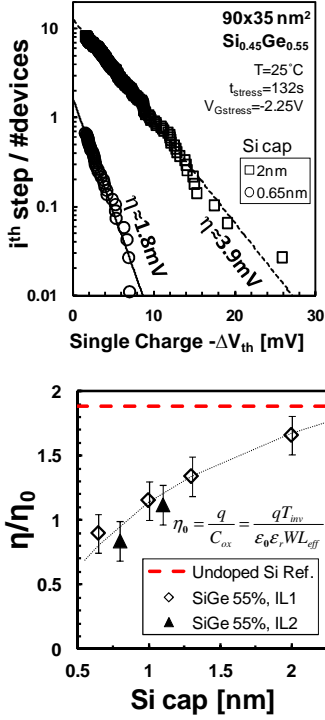
Fig. 6: Weighted CCDF plot of the \Delta V_{th} step heights observed on SiGe devices with two different Si cap thicknesses. The average \Delta V_{th} step height \eta is significantly reduced for the devices with the thinnest Si cap. Note also the reduced \langle N_T \rangle (lower y-axis intercept).
